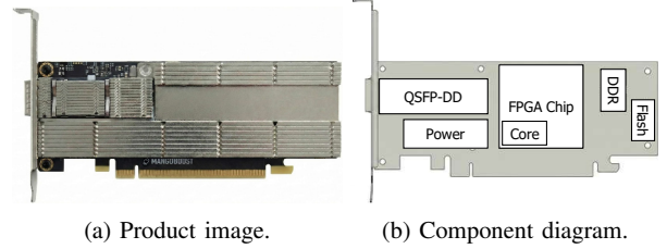
Fig. 5: DPU product image and internal component diagram.
