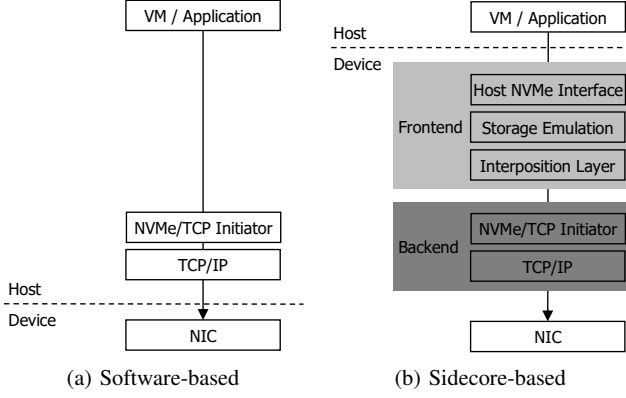
Fig. 3: Existing NVMe/TCP initiator solutions.
